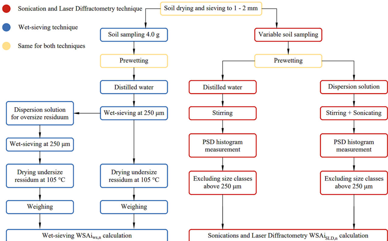
Fig. 2. Aggregate stability flow chart, simultaneous determination of WSAi by Wet-sieving and by the Sonication and Laser Diffraction approaches.
