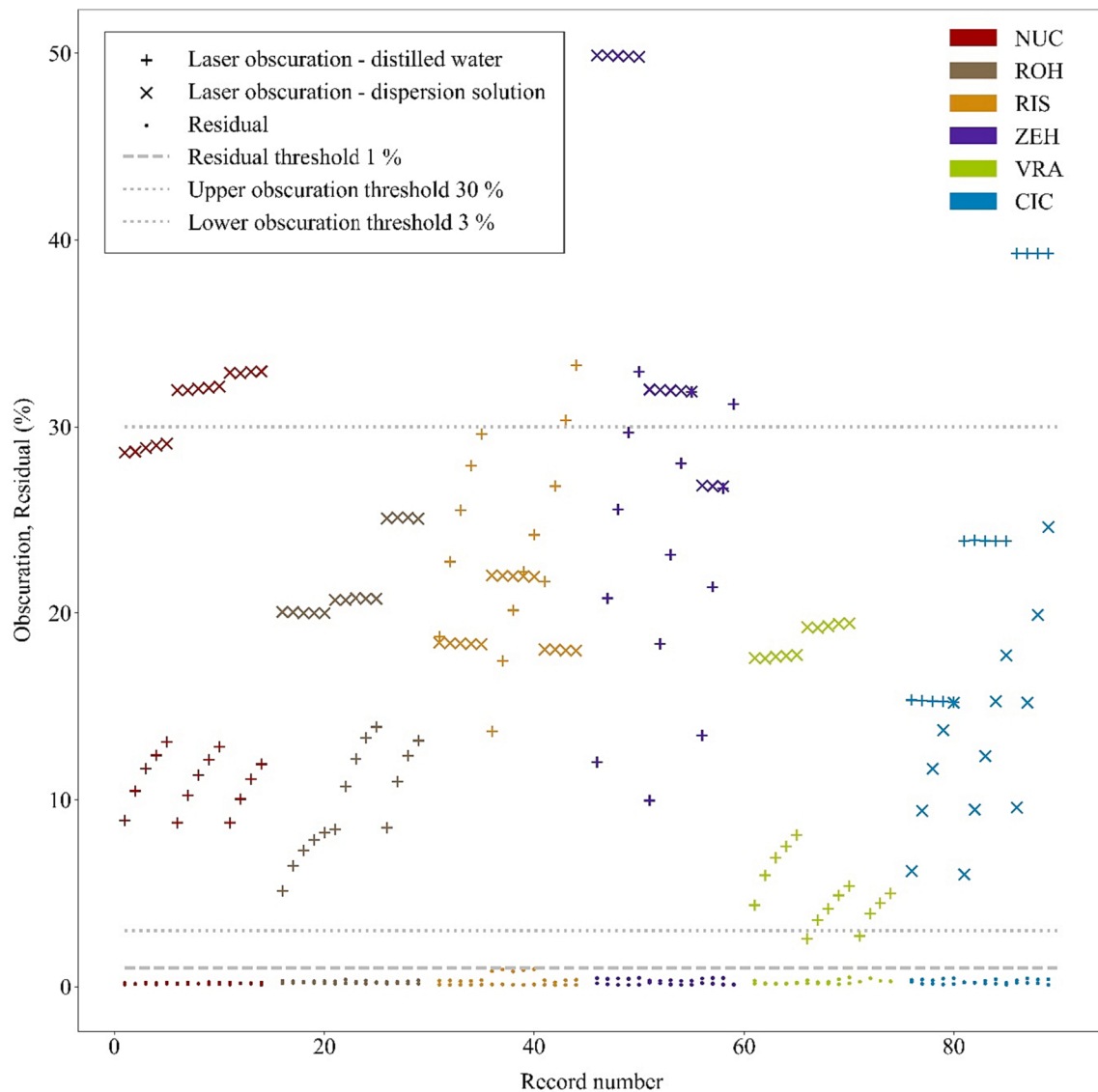
Fig. 4. Adjustment of the measured data, the cross sign stands for the degree of obscuration for the measurements in the dispersion solution, the plus sign stands for the degree of obscuration for the measurements in distilled water, the grey dashed line is the upper limit for the residuals, the grey dotted lines are the lower and upper recommended limits for the obscuration. The soil samples are represented by different colours.
