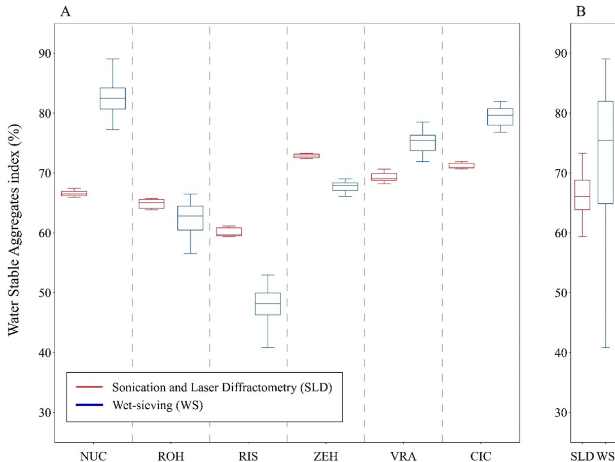
Fig. 5. Distribution of water stable aggregates indexes obtained by SLD (red) and by WS (blue) for different soils. Fig. A shows the WSAi for each soil obtained either by wet-sieving or by laser diffraction, Fig. B shows all WSAi if combined (points – outliers, bottom line – Q1, middle line – median, top line – Q3, interquartile range IQR = Q3 – Q1, upper whiskers = Q3 + 1.5(IQR), lower whiskers = Q1 – 1.5(IQR).
