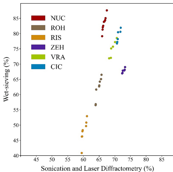
Fig. 6. Scatter diagram of WSAi measured by Sonication and Laser Diffraction (SLD) and Wet-sieving (WS) methods. Datapoints represent the calculated WSAi.
