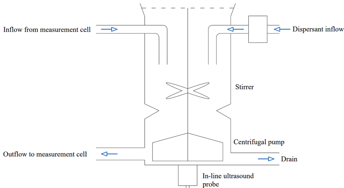
Fig. 1. Scheme of automated Hydro LV (adapted from Malvern, 2013).
