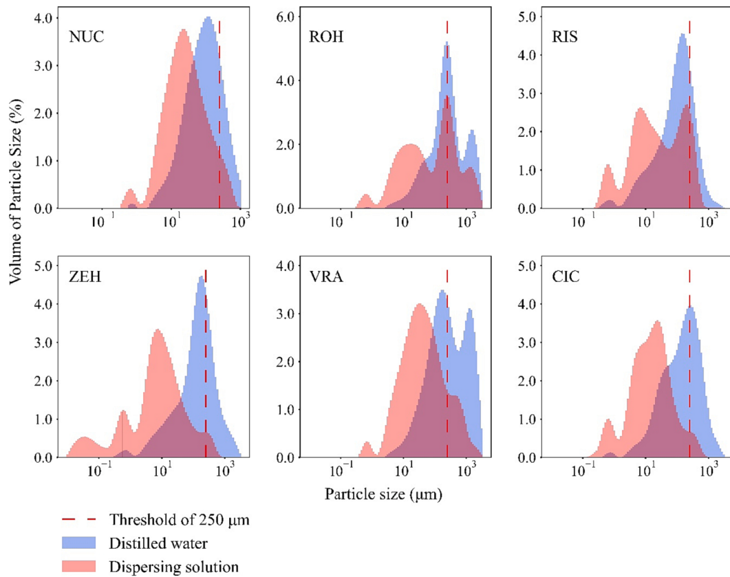
Fig. 3. Histograms of the particle and aggregate size distribution of the tested soils obtained during the sonication and laser diffraction technique, aggregates disrupted in water (blue), aggregates disrupted in the dispersion solution (red). The threshold line separates the particles above 250 \mu\text{m} that are not included in the WSAi calculation.
